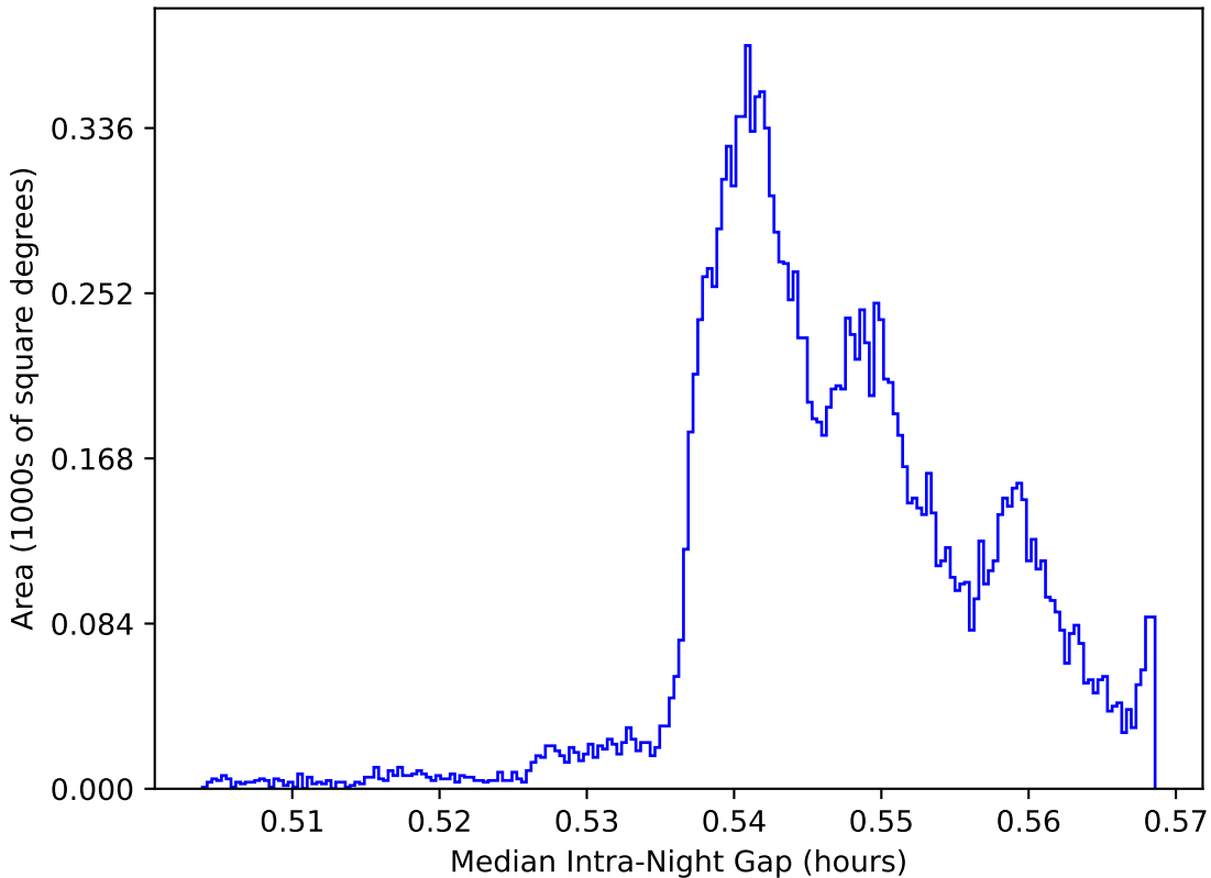
ddf_acor_sf15_lsf20_lsr20_v3.4_10yrs WFD: Median Intra-Night Gap
