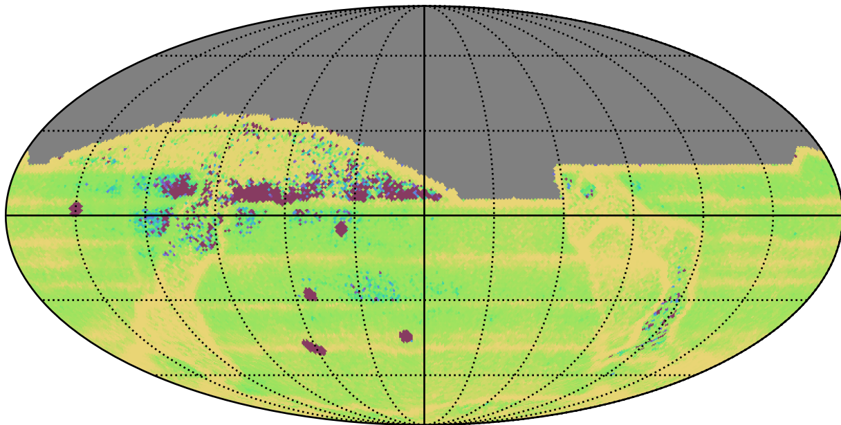
ddf_acor_sf15_lsf20_lsr20_v3.4_10yrs All sky: Median Intra-Night Gap
