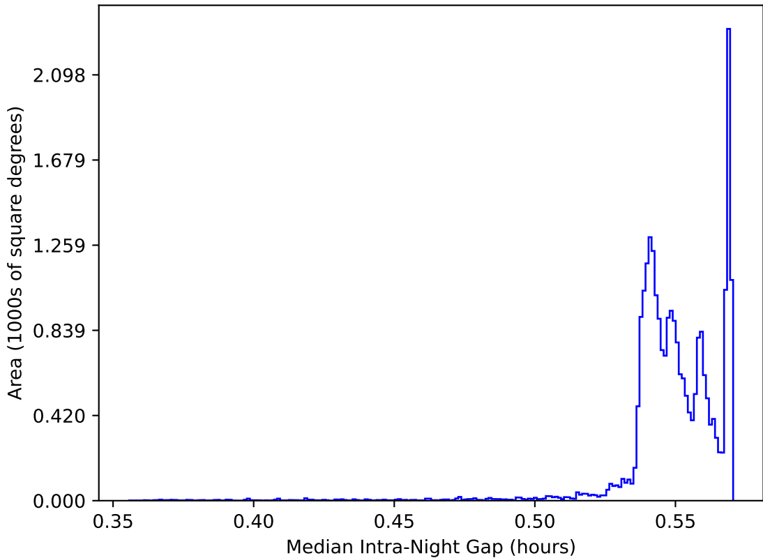
ddf_acor_sf15_lsf20_lsr20_v3.4_10yrs All sky: Median Intra-Night Gap
