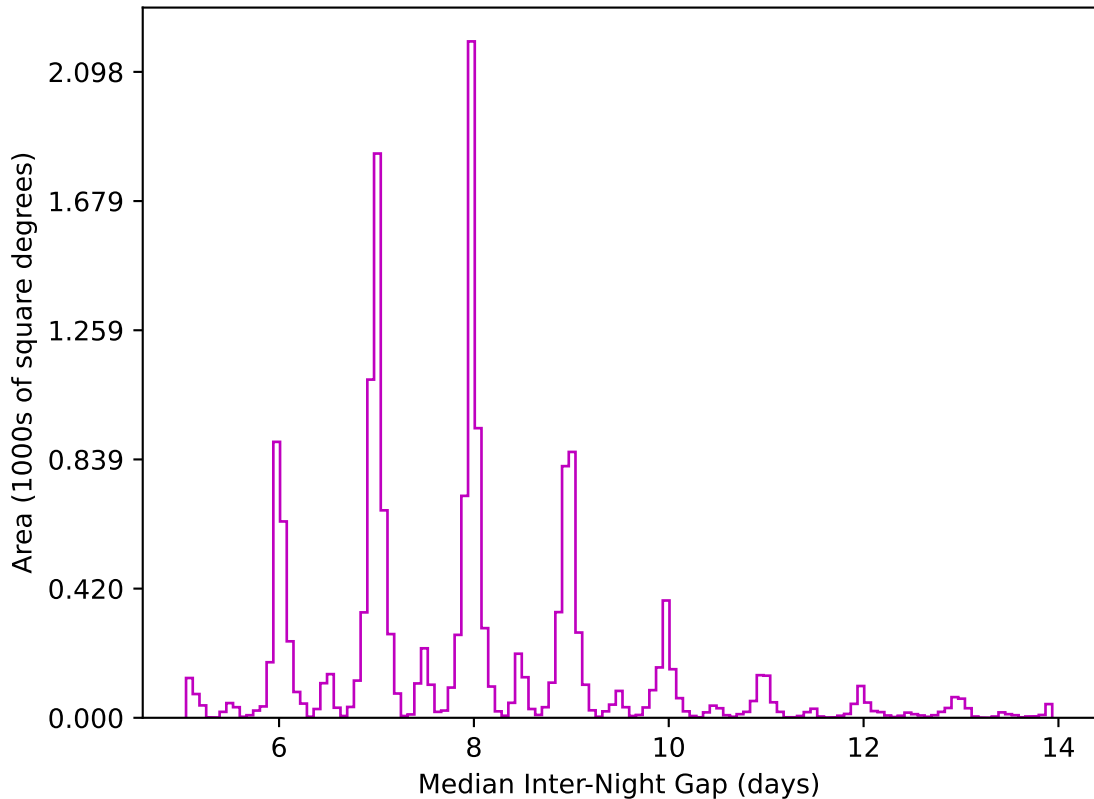
ddf_acor_sf15_lsf20_lsr20_v3.4_10yrs WFD z band: Median Inter-Night Gap
