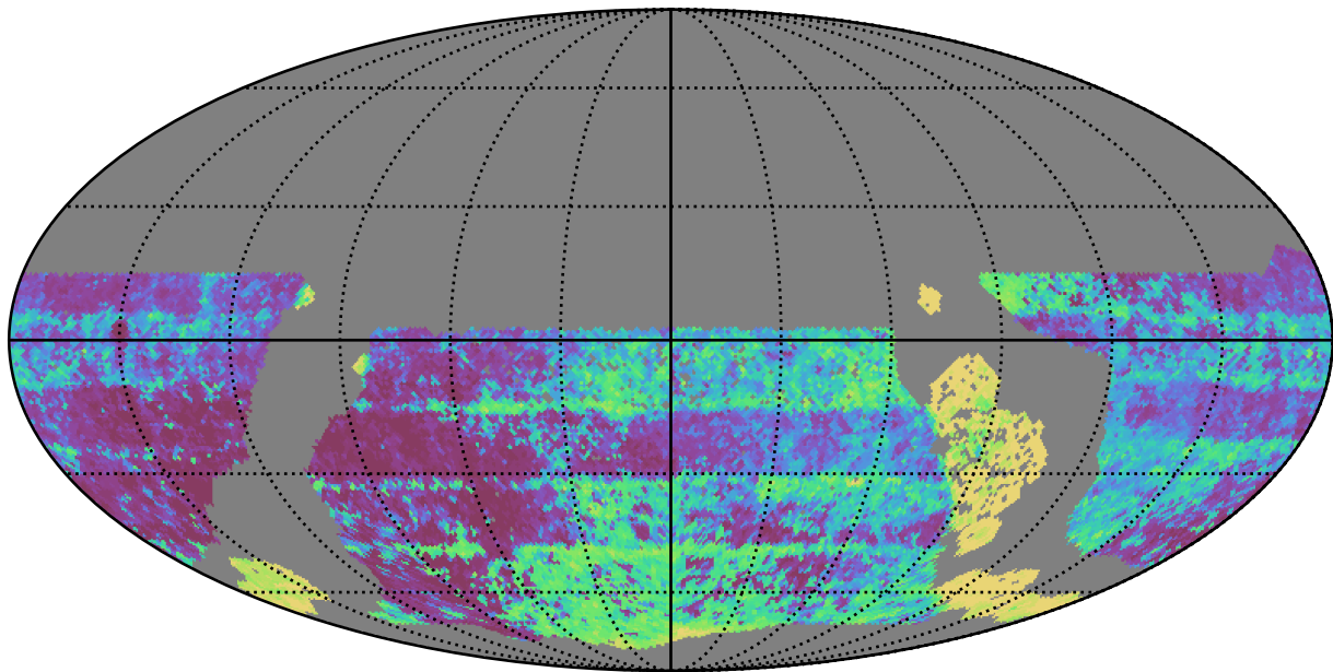
ddf_acor_sf15_lsf20_lsr20_v3.4_10yrs WFD y band: Median Inter-Night Gap
