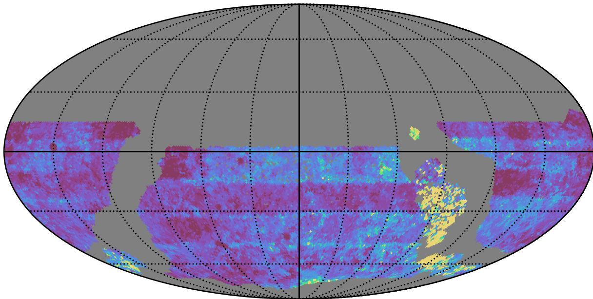
ddf_acor_sf15_lsf20_lsr20_v3.4_10yrs WFD u band: Median Inter-Night Gap
