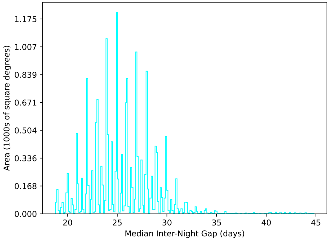
ddf_acor_sf15_lsf20_lsr20_v3.4_10yrs WFD u band: Median Inter-Night Gap
