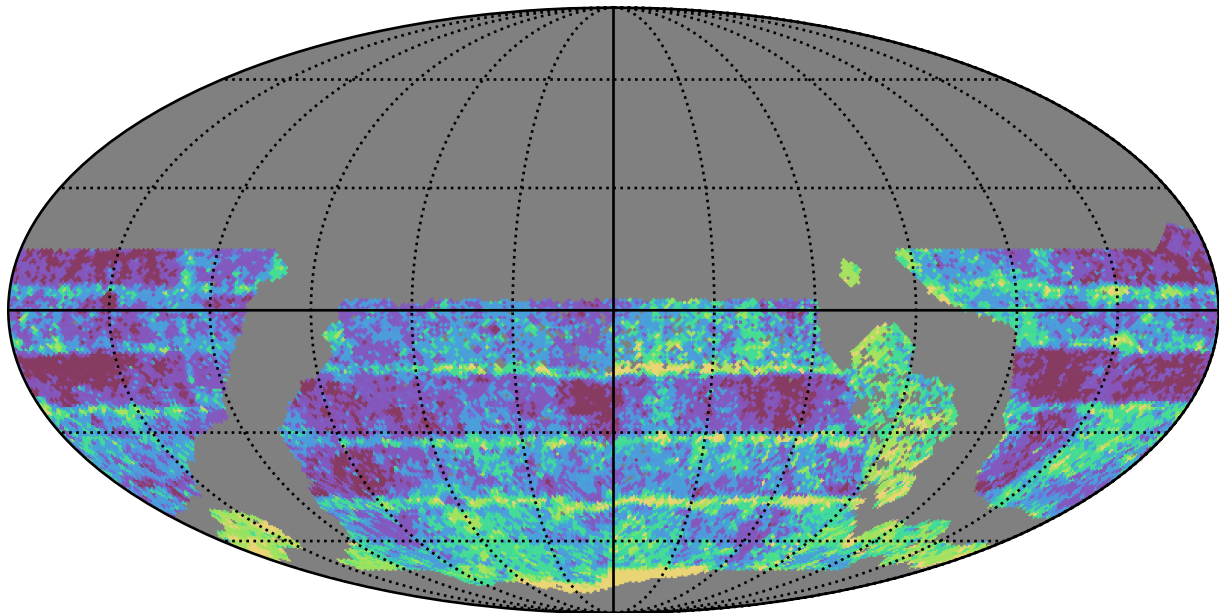
ddf_acor_sf15_lsf20_lsr20_v3.4_10yrs WFD r band: Median Inter-Night Gap
