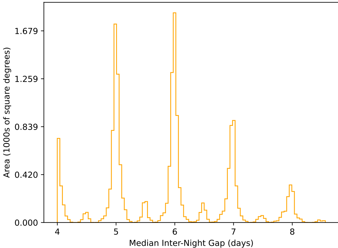
ddf_acor_sf15_ls20_lsr20_v3.4_10yrs WFD r band: Median Inter-Night Gap
