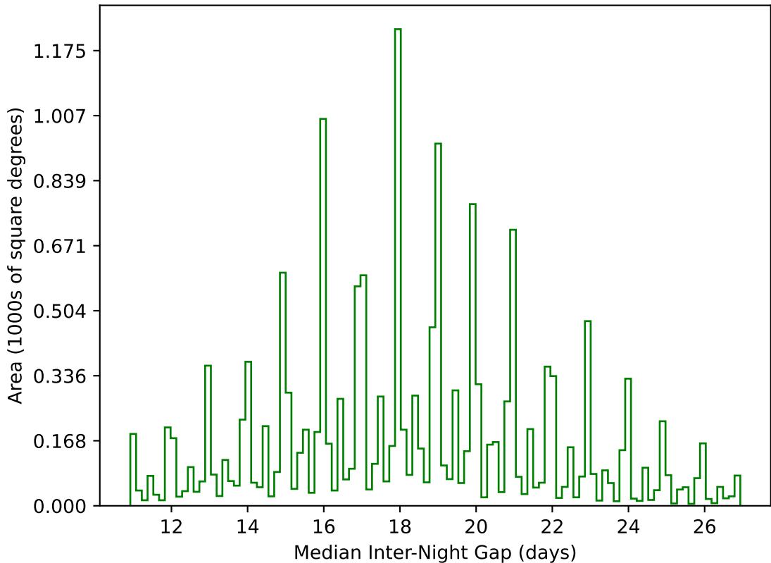
ddf_acor_sf15_lsf20_lsr20_v3.4_10yrs WFD g band: Median Inter-Night Gap
