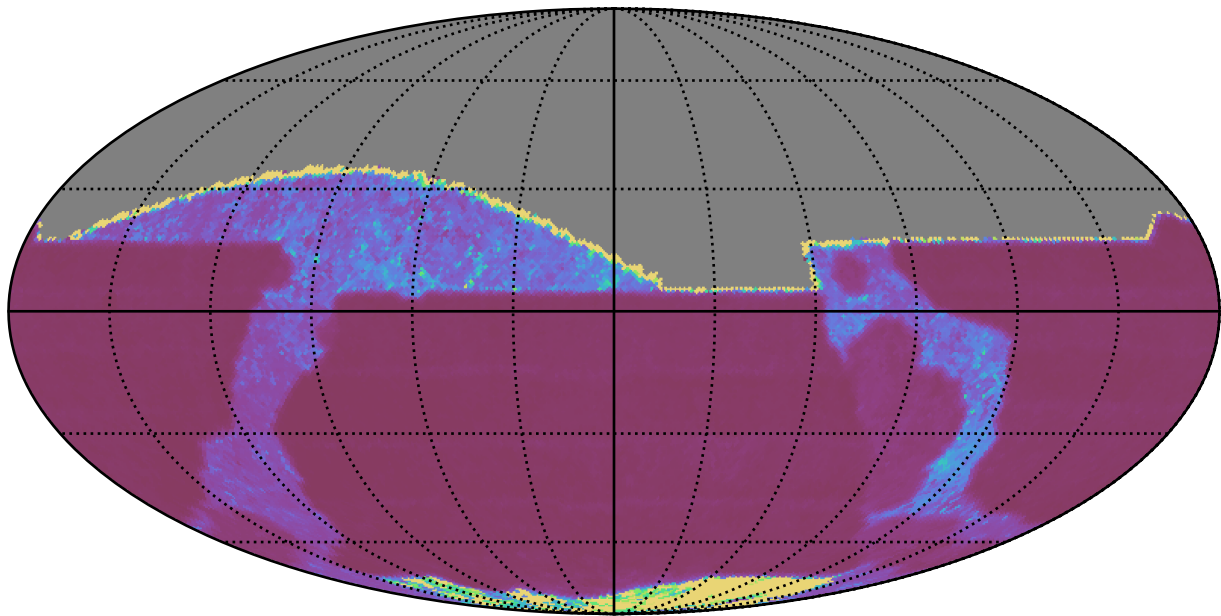
ddf_acor_sf15_lsf20_lsr20_v3.4_10yrs All sky z band: Median Inter-Night Gap
