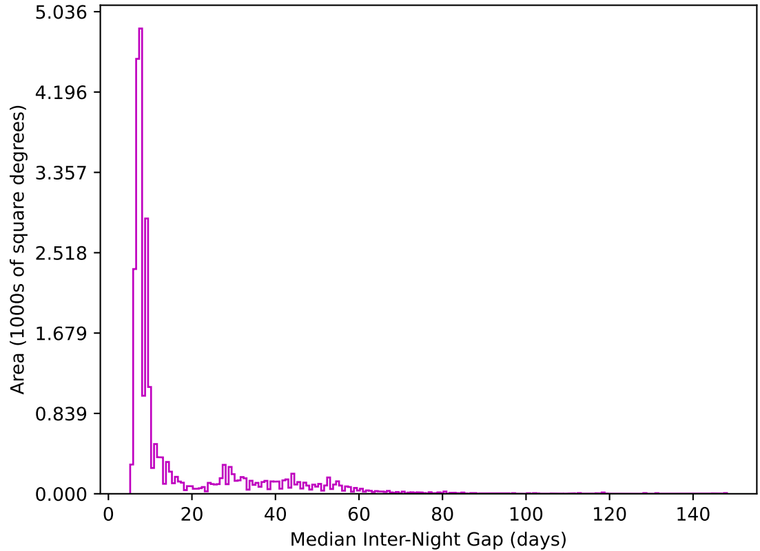
ddf_acor_sf15_lsf20_lsr20_v3.4_10yrs All sky z band: Median Inter-Night Gap
