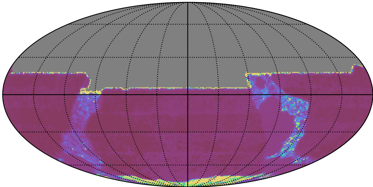
ddf_acor_sf15_lsf20_lsr20_v3.4_10yrs All sky y band: Median Inter-Night Gap
