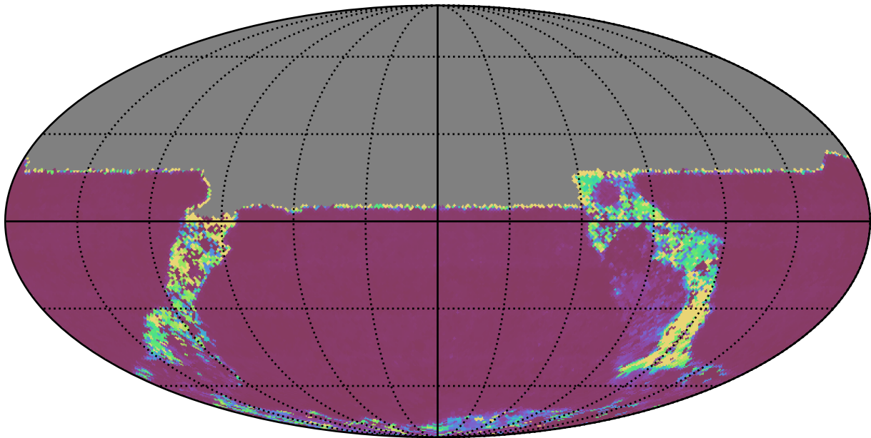
ddf_acor_sf15_lsf20_lsr20_v3.4_10yrs All sky u band: Median Inter-Night Gap
