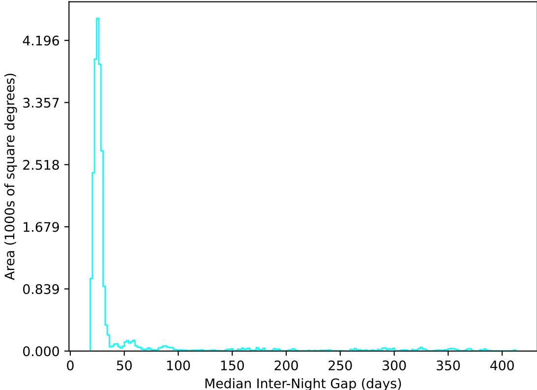
ddf_acor_sf15_lsf20_lsr20_v3.4_10yrs All sky u band: Median Inter-Night Gap
