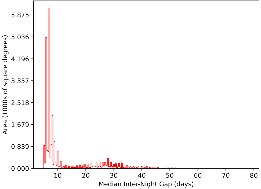
ddf_acor_sf15_lsf20_lsr20_v3.4_10yrs All sky i band: Median Inter-Night Gap
