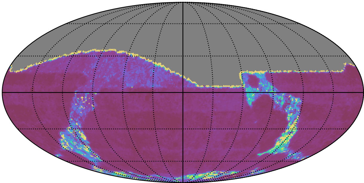
ddf_acor_sf15_lsf20_lsr20_v3.4_10yrs All sky g band: Median Inter-Night Gap
