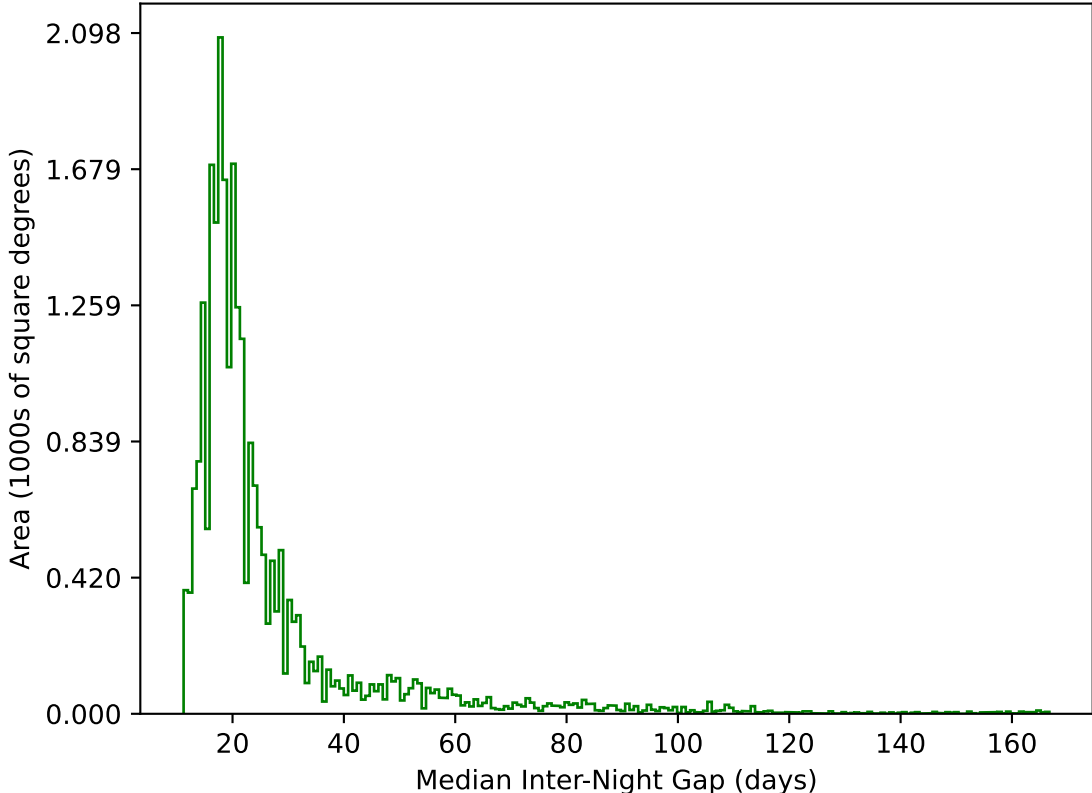
ddf_acor_sf15_lsf20_lsr20_v3.4_10yrs All sky g band: Median Inter-Night Gap
