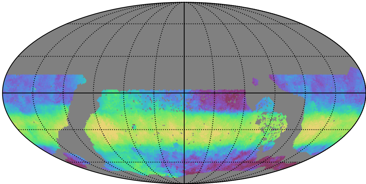
ddf_acor_sf15_lsf20_lsr20_v3.4_10yrs WFD z band: Median HA
