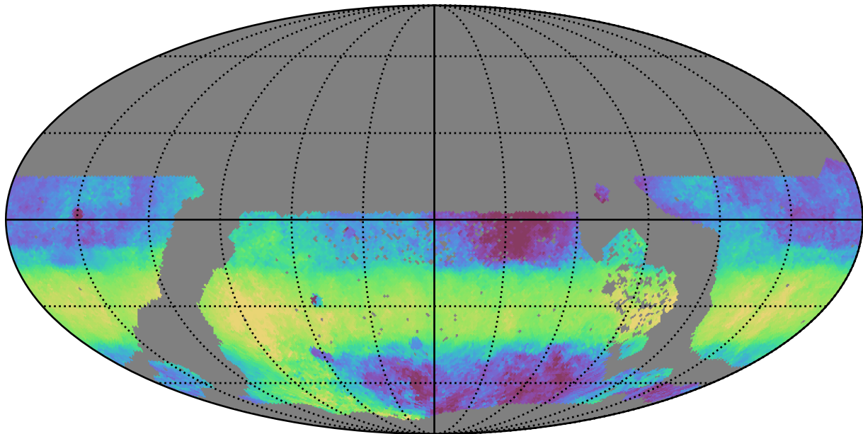
ddf_acor_sf15_lsf20_lsr20_v3.4_10yrs WFD y band: Median HA
