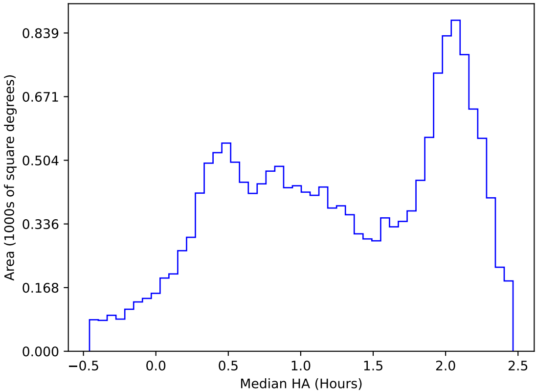
ddf_acor_sf15_lsf20_lsr20_v3.4_10yrs WFD y band: Median HA
