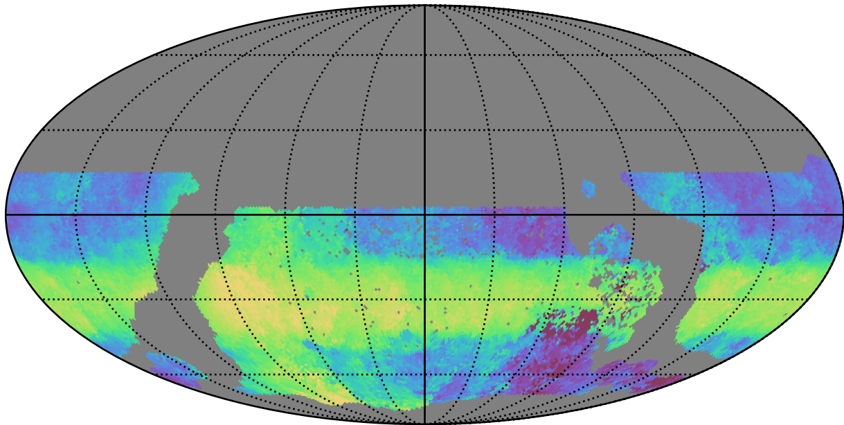
ddf_acor_sf15_lsf20_lsr20_v3.4_10yrs WFD u band: Median HA
