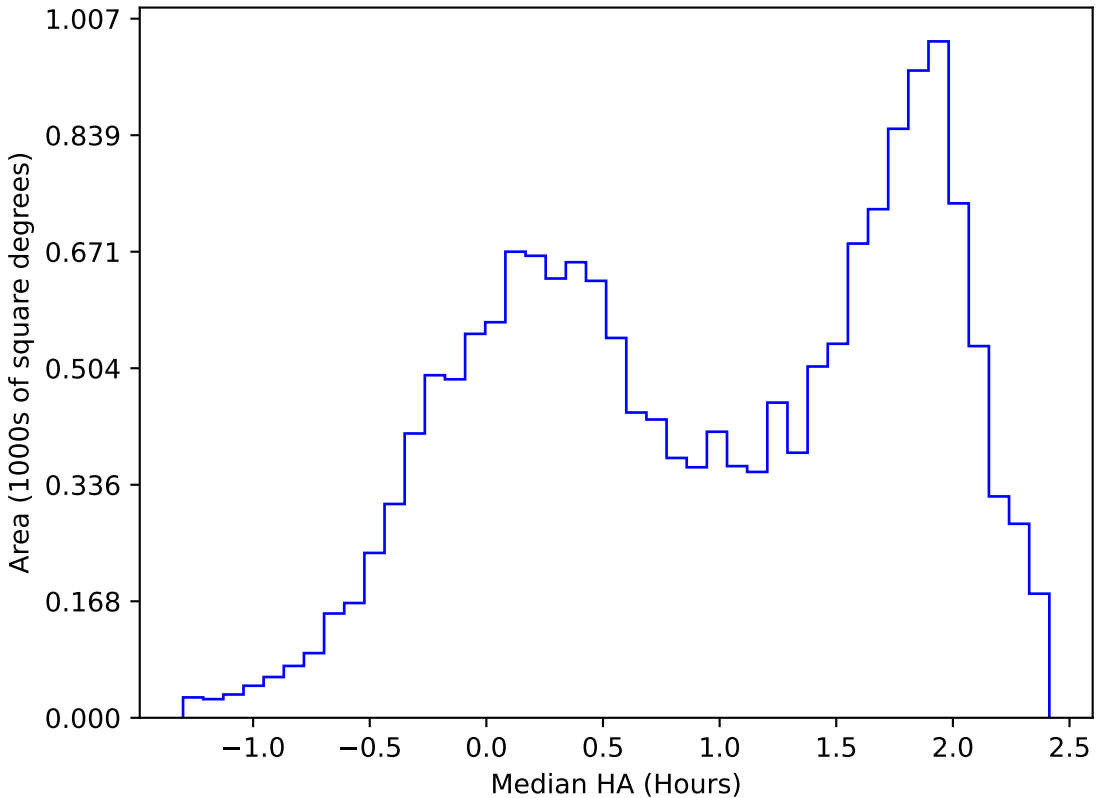
ddf_acor_sf15_lsf20_lsr20_v3.4_10yrs WFD u band: Median HA
