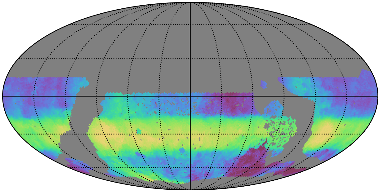
ddf_acor_sf15_lsf20_lsr20_v3.4_10yrs WFD r band: Median HA
