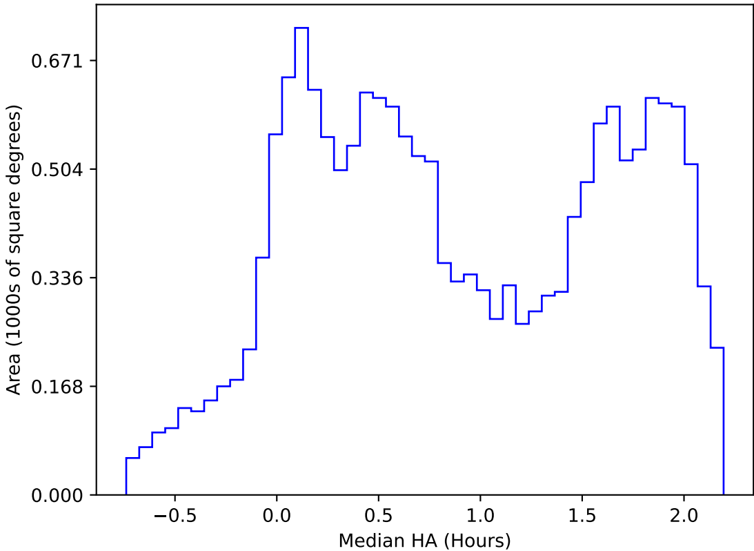
ddf_acor_sf15_lsf20_lsr20_v3.4_10yrs WFD r band: Median HA
