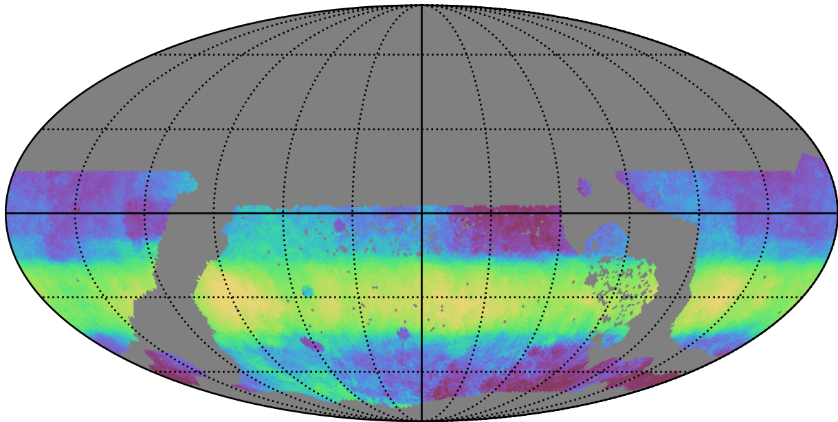
ddf_acor_sf15_lsf20_lsr20_v3.4_10yrs WFD i band: Median HA
