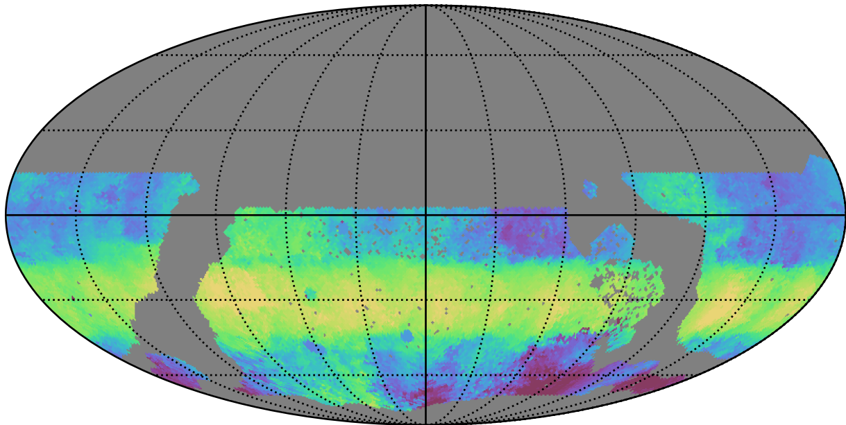
ddf_acor_sf15_lsf20_lsr20_v3.4_10yrs WFD g band: Median HA
