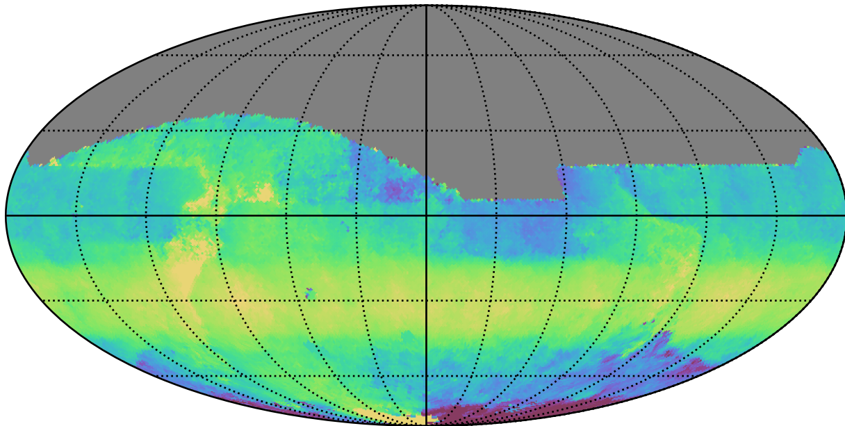
ddf_acor_sf15_lsf20_lsr20_v3.4_10yrs All sky z band: Median HA
