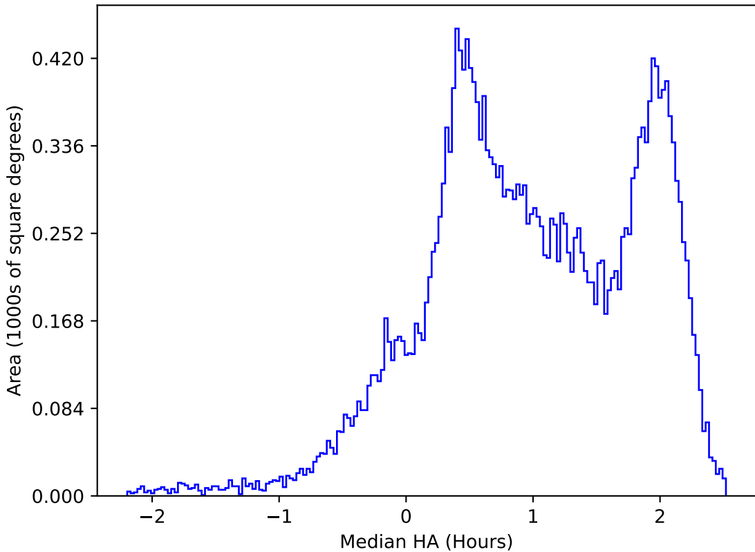
ddf_acor_sf15_lsf20_lsr20_v3.4_10yrs All sky z band: Median HA
