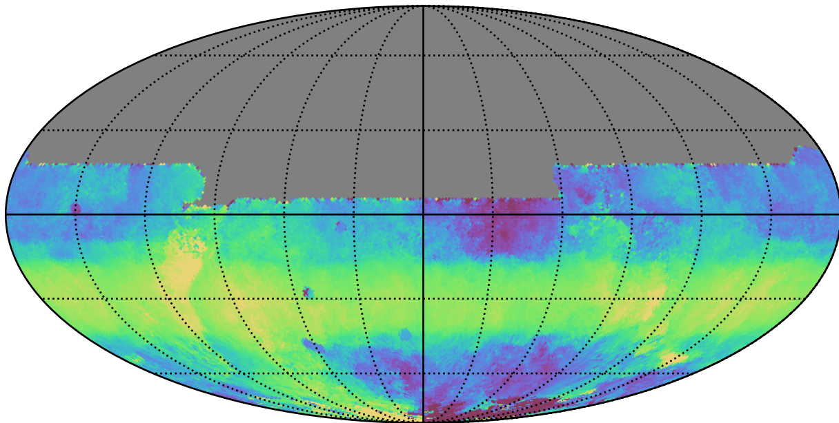
ddf_acor_sf15_lsf20_lsr20_v3.4_10yrs All sky y band: Median HA
