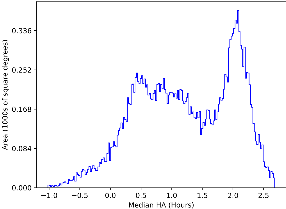
ddf_acor_sf15_ls20_lsr20_v3.4_10yrs All sky y band: Median HA
