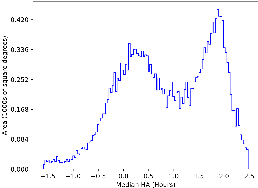
ddf_acor_sf15_lsf20_lsr20_v3.4_10yrs All sky u band: Median HA
