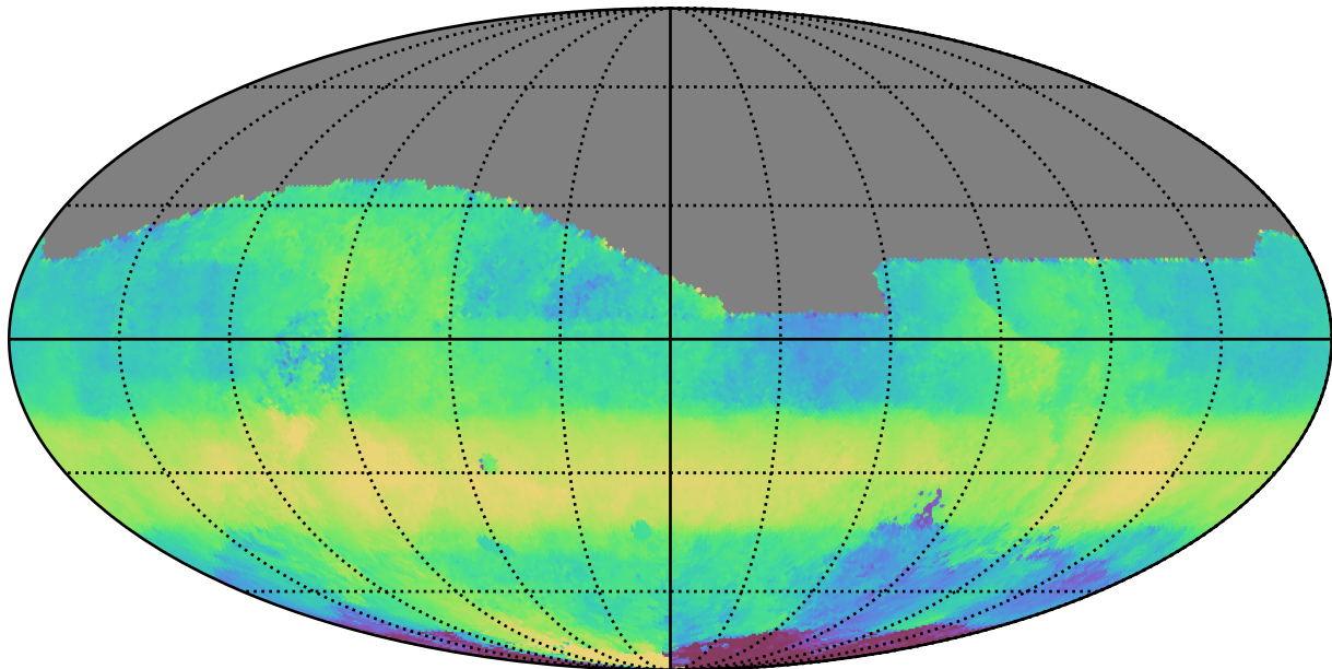
ddf_acor_sf15_lsf20_lsr20_v3.4_10yrs All sky r band: Median HA
