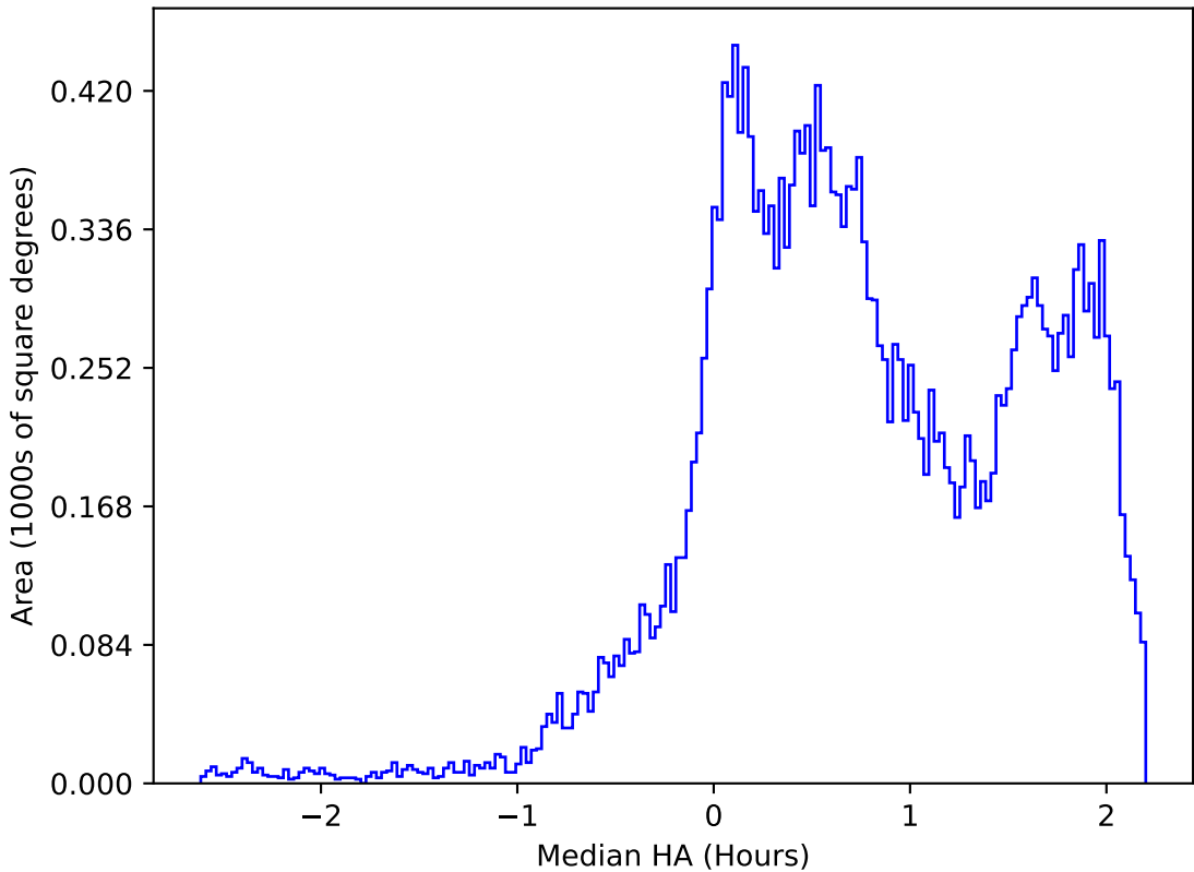
ddf_acor_sf15_lsf20_lsr20_v3.4_10yrs All sky r band: Median HA
