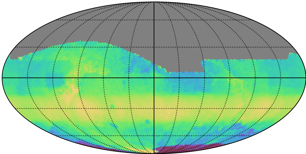
ddf_acor_sf15_lsf20_lsr20_v3.4_10yrs All sky i band: Median HA
