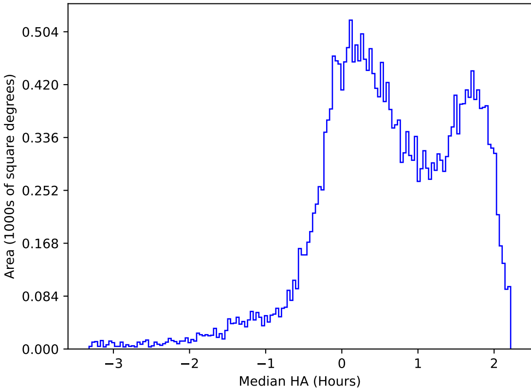
ddf_acor_sf15_lsf20_lsr20_v3.4_10yrs All sky g band: Median HA
