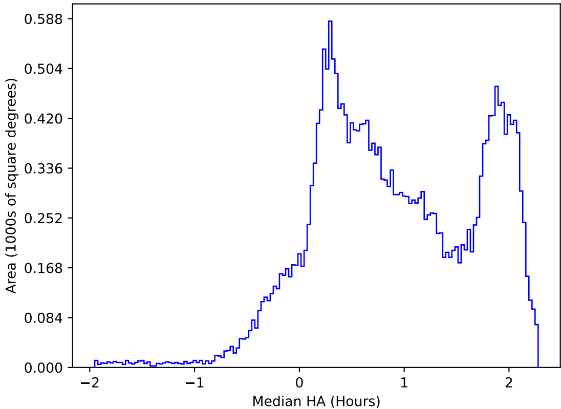
ddf_acor_sf15_lsf20_lsr20_v3.4_10yrs All sky all bands: Median HA
