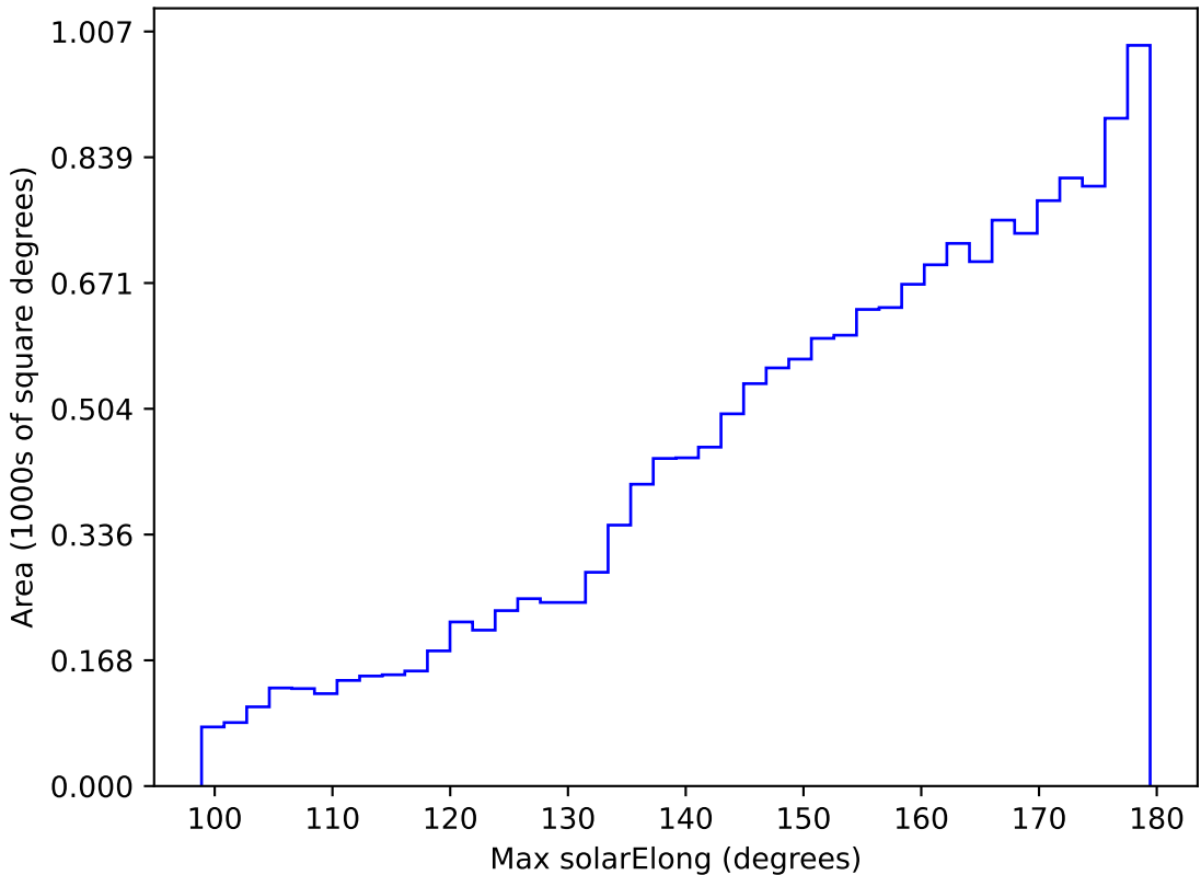
ddf_acor_sf15_lsf20_lsr20_v3.4_10yrs WFD z band: Max solarElong
