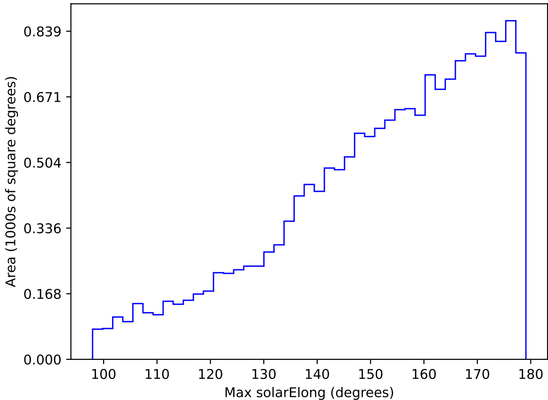
ddf_acor_sf15_lsf20_lsr20_v3.4_10yrs WFD u band: Max solarElong
