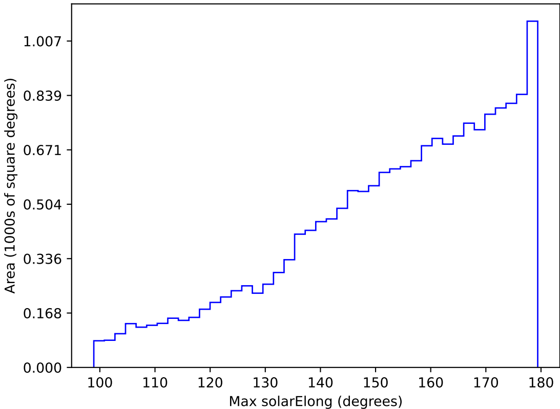
ddf_acor_sf15_lsf20_lsr20_v3.4_10yrs WFD i band: Max solarElong
