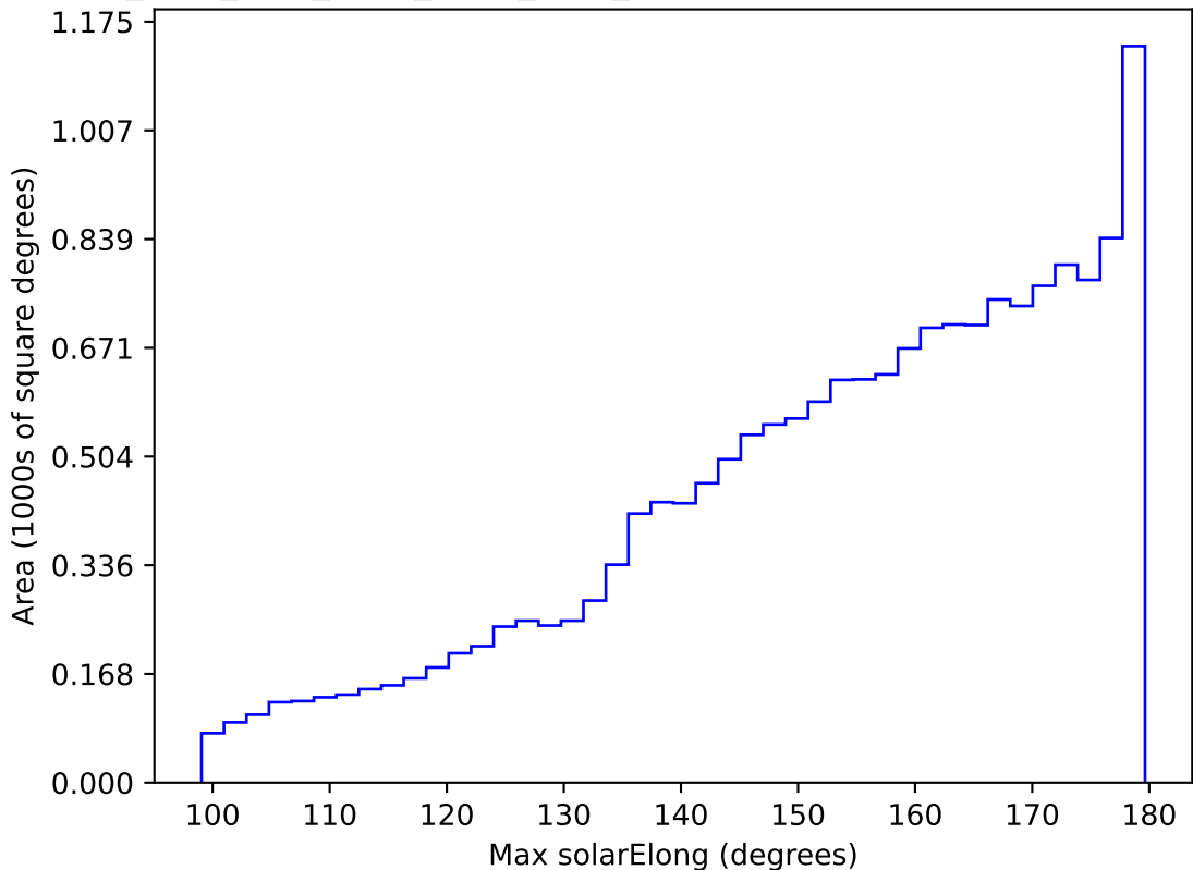
ddf_acor_sf15_lsf20_lsr20_v3.4_10yrs WFD all bands: Max solarElong
