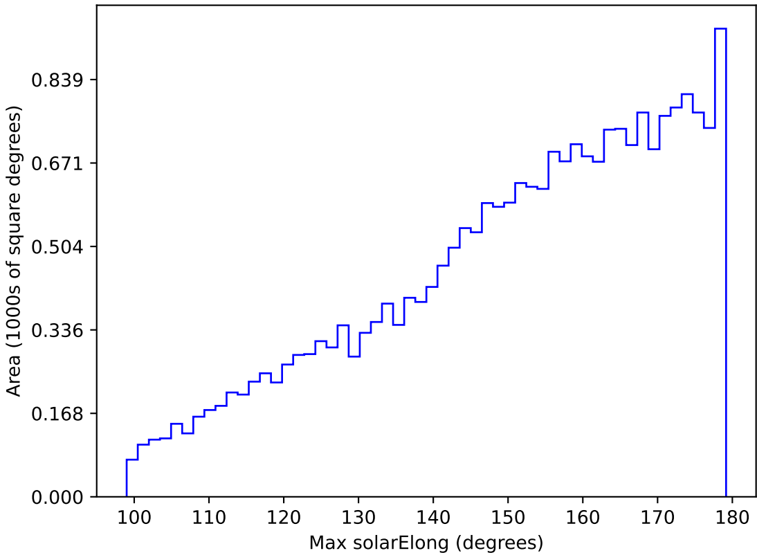
ddf_acor_sf15_lsf20_lsr20_v3.4_10yrs All sky y band: Max solarElong
