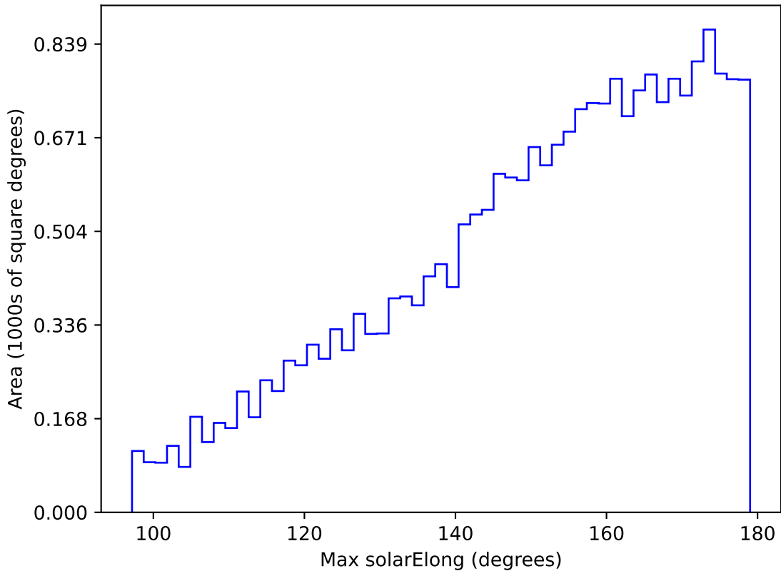
ddf_acor_sf15_lsf20_lsr20_v3.4_10yrs All sky u band: Max solarElong
