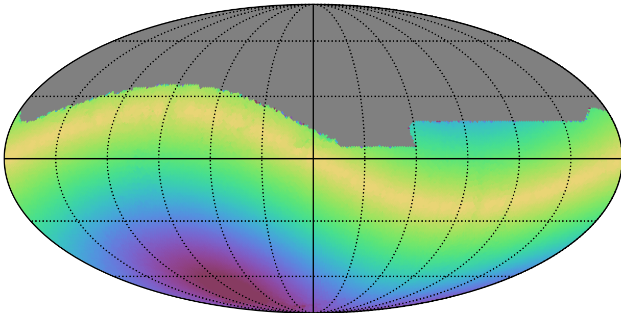
ddf_acor_sf15_lsf20_lsr20_v3.4_10yrs All sky r band: Max solarElong
