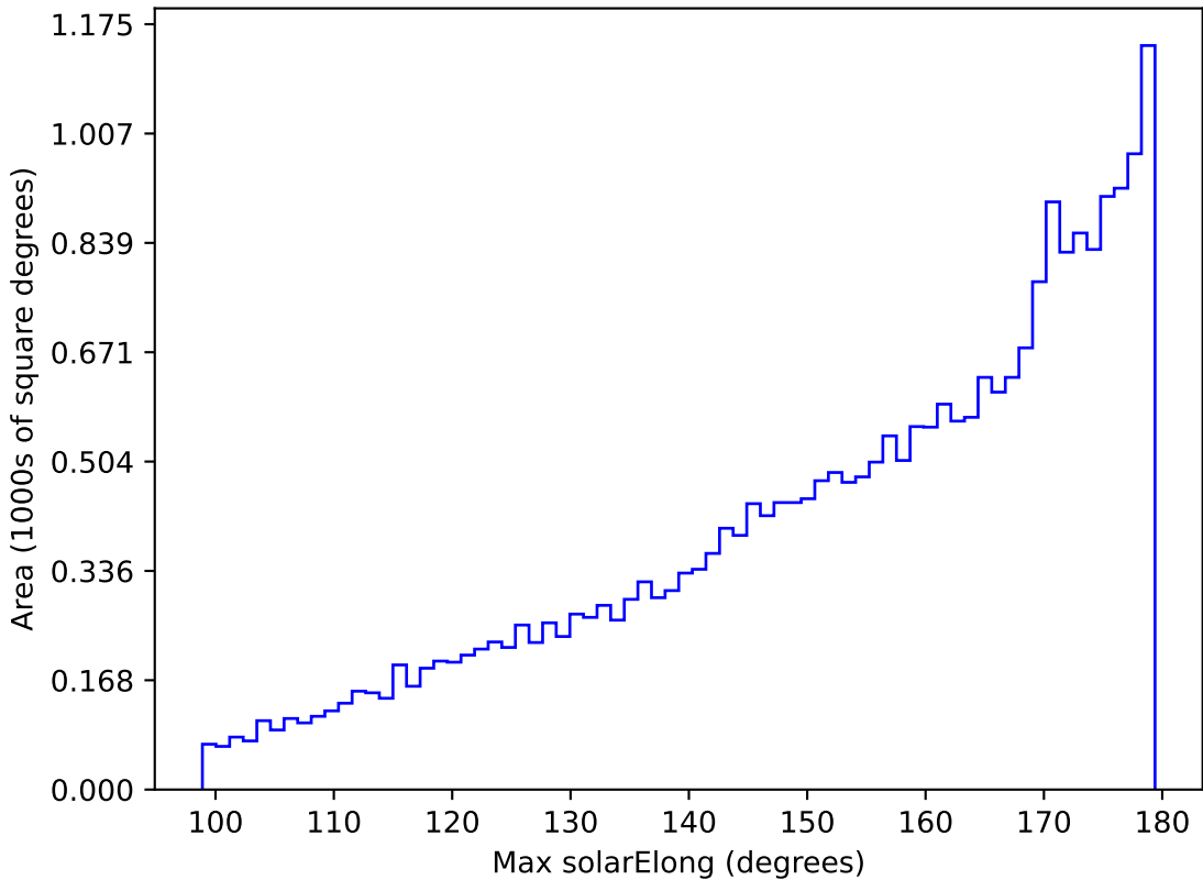
ddf_acor_sf15_lsf20_lsr20_v3.4_10yrs All sky i band: Max solarElong
