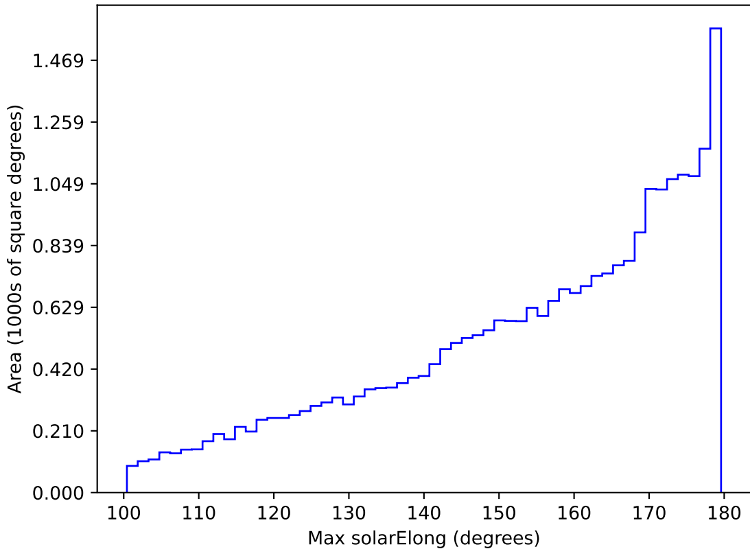
ddf_acor_sf15_lsf20_lsr20_v3.4_10yrs All sky all bands: Max solarElong
