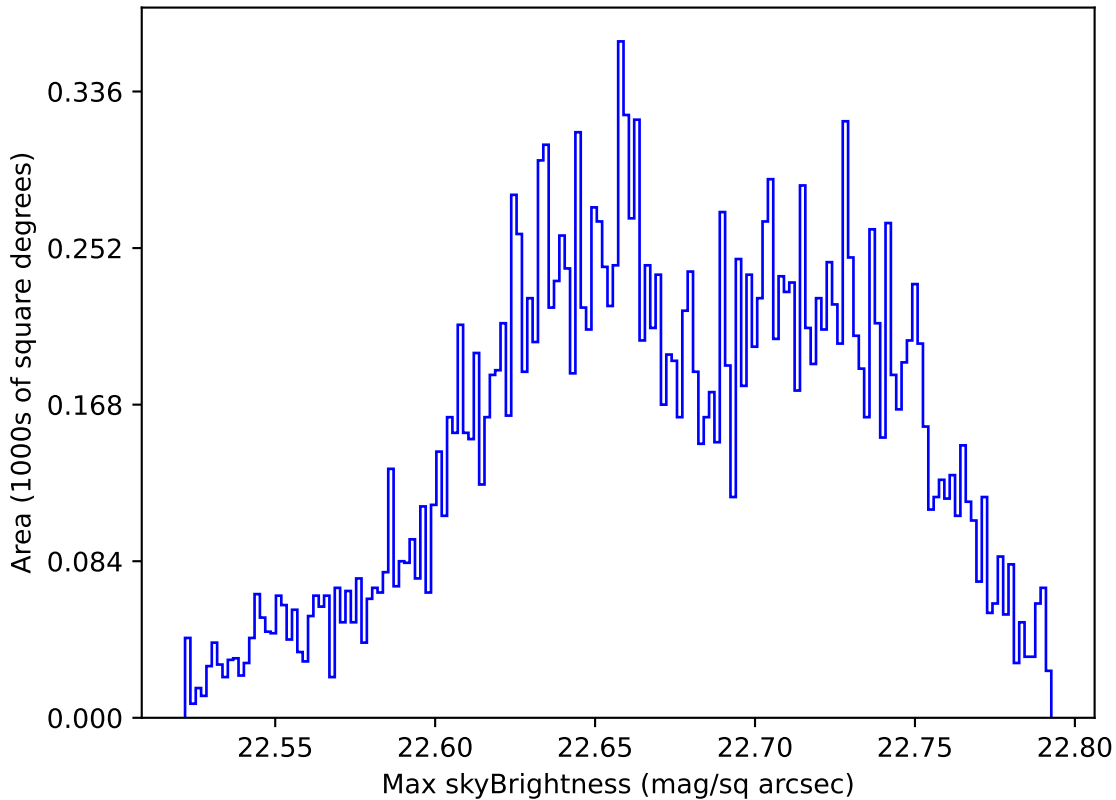
ddf_acor_sf15_lsf20_lsr20_v3.4_10yrs Yr 1 u band: Max skyBrightness
