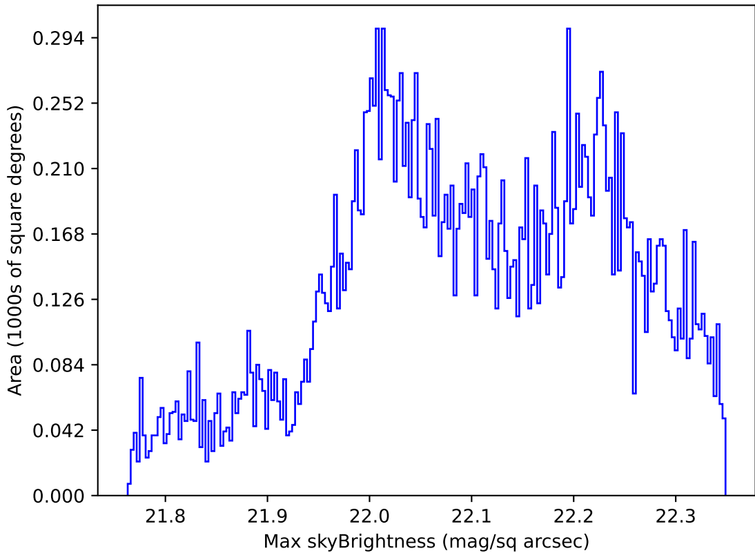
ddf_acor_sf15_lsf20_lsr20_v3.4_10yrs Yr 1 g band: Max skyBrightness
