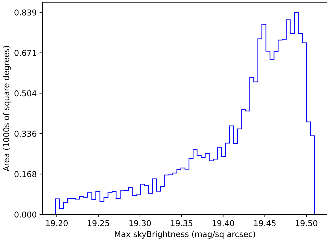
ddf_acor_sf15_lsf20_lsr20_v3.4_10yrs WFD z band: Max skyBrightness
