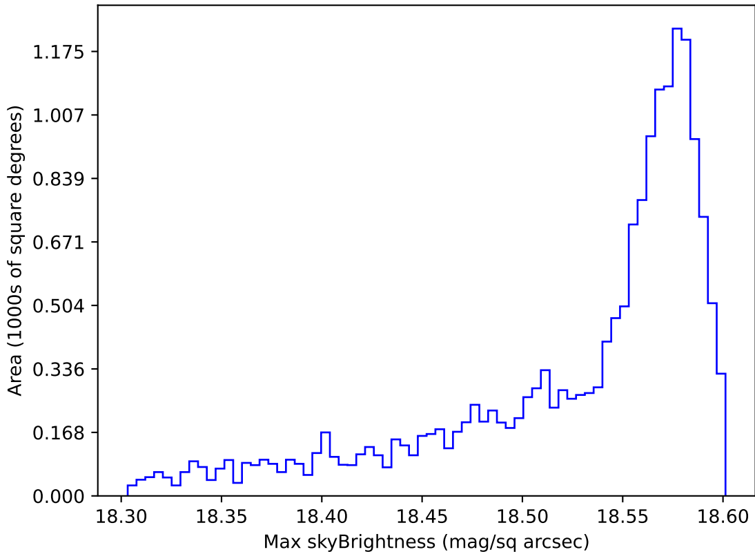
ddf_acor_sf15_lsf20_lsr20_v3.4_10yrs WFD y band: Max skyBrightness
